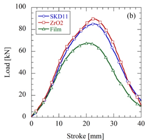
図5 Punch load-stroke curve : punch speed (a)200mm/s ,(b)60mm/s
