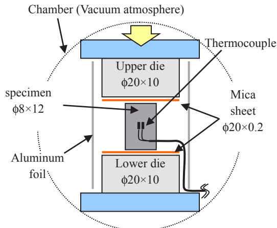
図1 Schematic illustration of experimental apparatus for compression test
