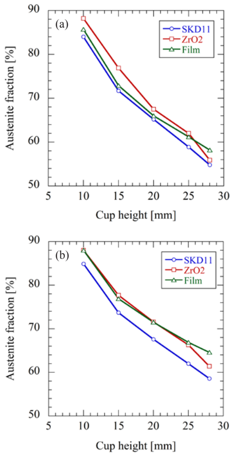
図6 Effect of tools on austenite fraction : punch speed (a)200mm/s, (b)60mm/s
