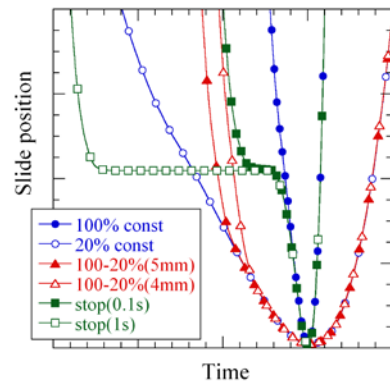
図 9 Various slide motion patterns used in this study.
