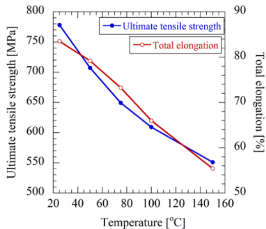
図3 Mechanical property of specimen
