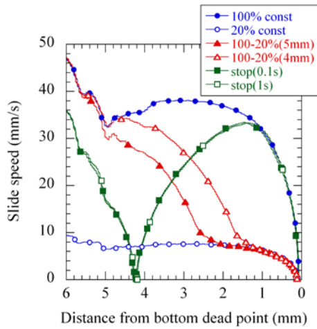
図 10 Slide speed of various slide motion patterns used in this study
