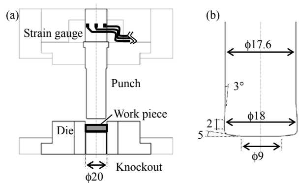
図 8 Schematic illustrations of (a) cross section of experimental apparatus and (b) front edge of punch
