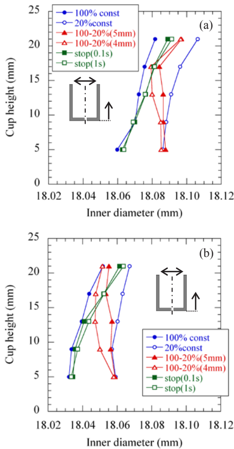
図 11 Variation of inner diameters of impact extruded cup : (a)experimental, (b)calculated
