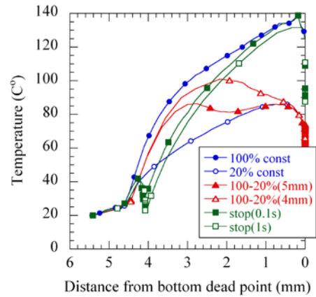
図 12 Effect of slide motion patterns on maximum work piece temperature (calculated)
