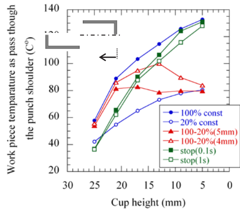
図 13 Distribution of work piece temperature as pass through the punch shoulder (calculated)
