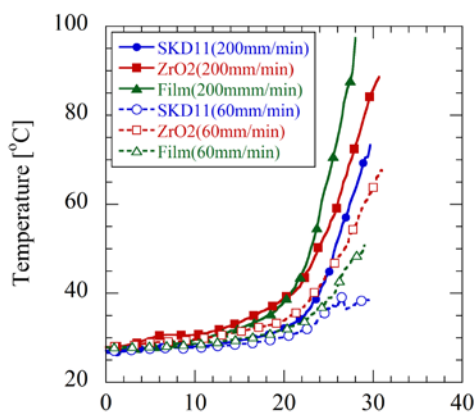
図4 Effect of tools and punch speed on blank temperature
